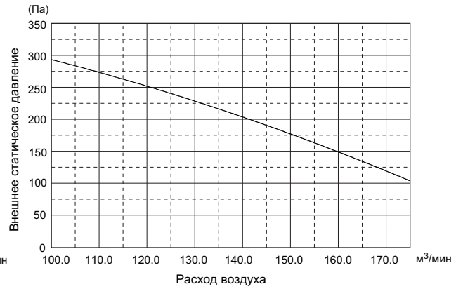
PEA-RP500GA
